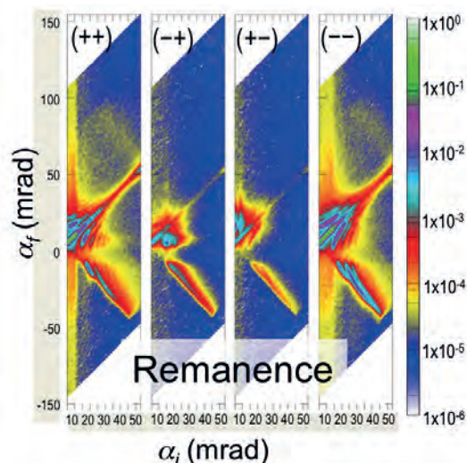
Fig. 3: Fe nat Fe 57 multilayer with 4.5 \mu\text{m} grating measured with full polarisation analysis with a large area ^3\text{He} neutron spin filter covering ~80% of the large PSD (400 mm x 400 mm).
