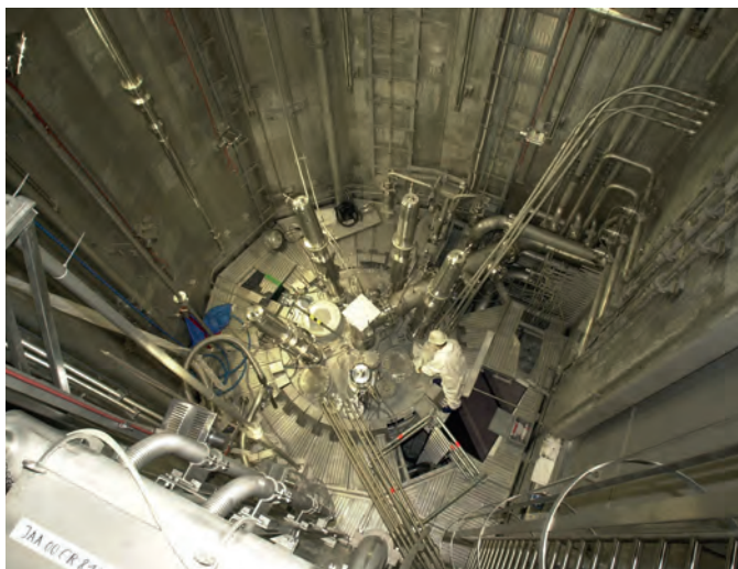
The reactor pool - still without water.
