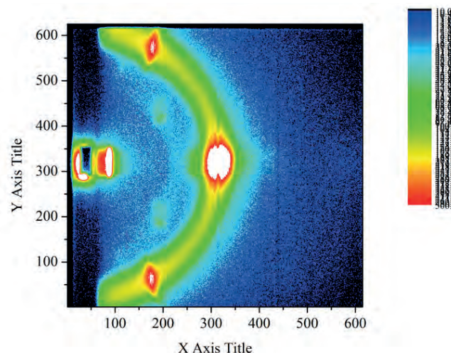
Fig. 4: GISANS soft-matter measurement with 10 \text{\AA} in 1200 seconds of C10E4 + Pep15Peo5 on a silicon surface in the hexagonal phase.
