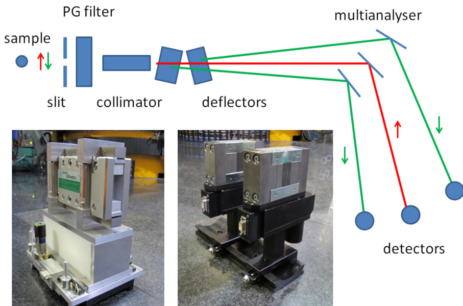
Fig. 1: The layout of the PUMA multianalyser polarisation analysis system. The collimator (left inset) and defectors (right inset) are equipped with micro-step motors for alignment.
