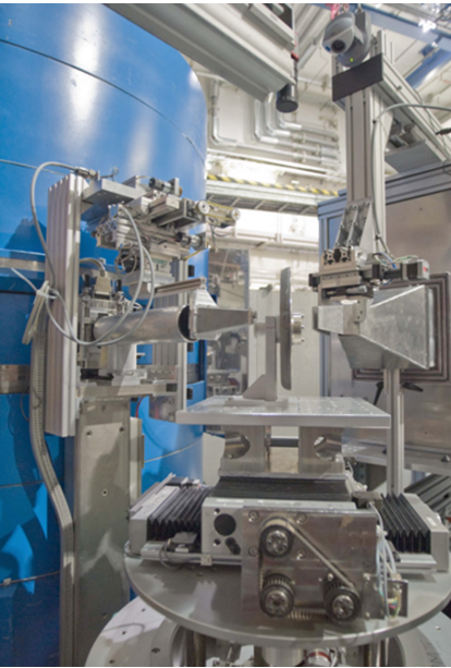
Fig. 1: STRESS-SPEC.
