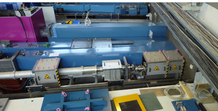
Fig. 1a: New mobile shielding installed at KWS-3.
