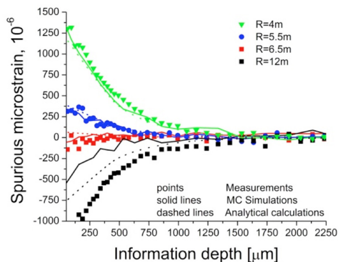
Fig. 2: Comparison of analytical calculations (dashed lines), MC simulations (solid lines) and experimental data (points) of spurious strains for the STRESS-SPEC diffractometer with bent Si(400) monochromator at different radii of curvature, R.
