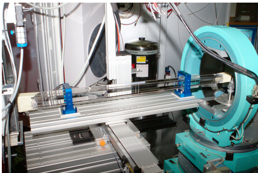
Fig. 2: Focussing guide of RESI.
