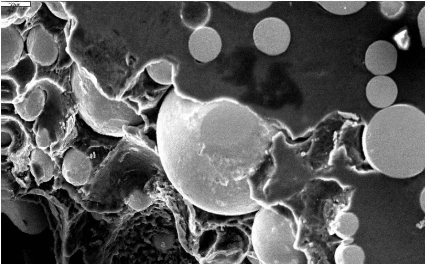
A scanning electron microscope picture of a cut-through disperse sample with Uranium-Molybdenum and aluminium.
