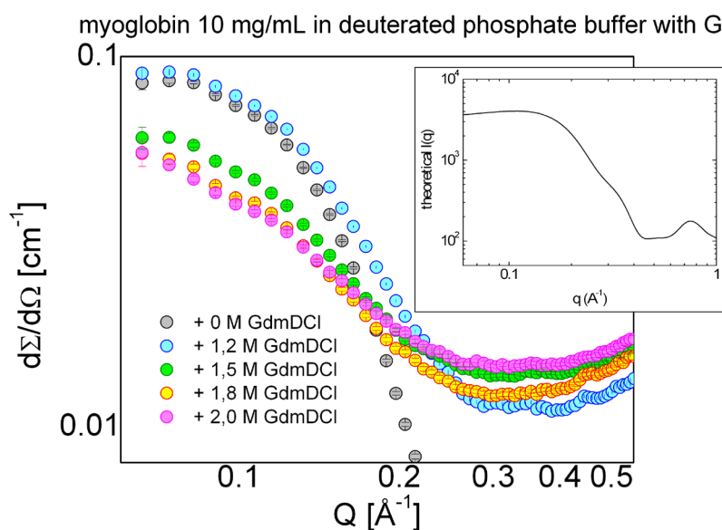
Fig.2: SANS patterns from a myoglobin protein in buffer solution for different amount of denaturing agent added. (In the courtesy of M.-S. Appavou)
