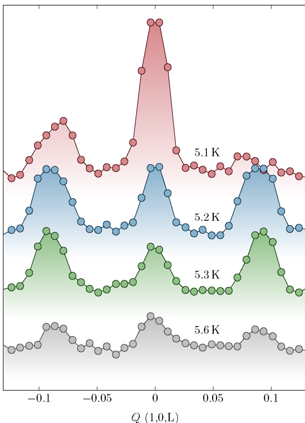
Figure 4: Temperature dependence of the commensurate CM (1,0,0) and incommensurate ICM-c* (1,0, ±0.085) magnetic peaks measured in antiferromagnetic superconductor \text{HoNi}_2\text{B}_2\text{C} with POLI-HEiDi. The y-axis is plotted in the logarithmic scale.
