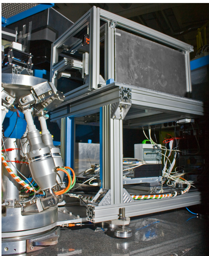
Figure 1: The sample position of MARIA with hexapod, ^3\text{He} -SEOP-analyzer and detector.
