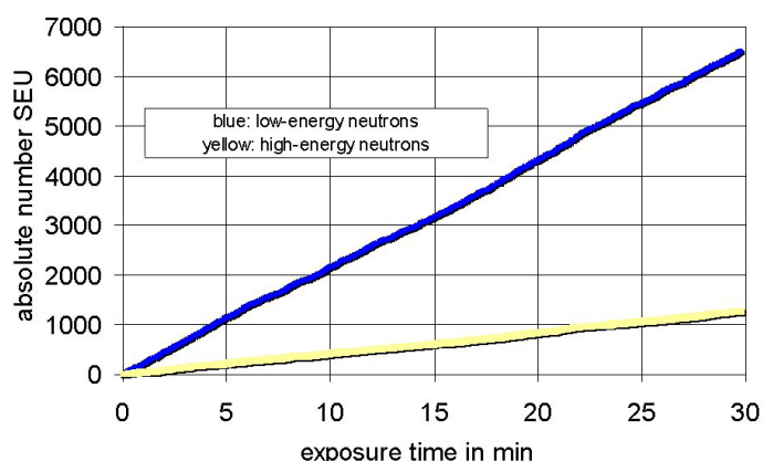
Figure 3: Neutron irradiation of a 4 Mbit SRAM device. Appearance of single-event-upsets (SEU) over a exposition period of 30 minutes. This correlates with 5,1 \cdot 10^{11} \text{ n/cm}^2 .
