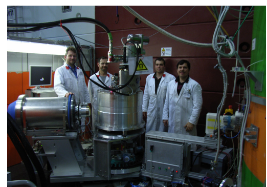
Figure 5: Technical feasibility study, test of the FRM II 7.5 T magnet on-site with POLI.
