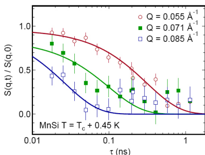
Figure 4: Spinecho data from MnSi above T_c . The life time of the fluctuations decreases quickly with increasing momentum transfer Q .
