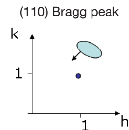
Figure 2: The basic principle of Larmor diffraction (LD), colour coded bragg intensity without LD (off) and with LD (on) (figure by K. Habicht, HZB). The modulation of the resolution ellipsoid increases the relative resolution \Delta d/d by a factor 100.
