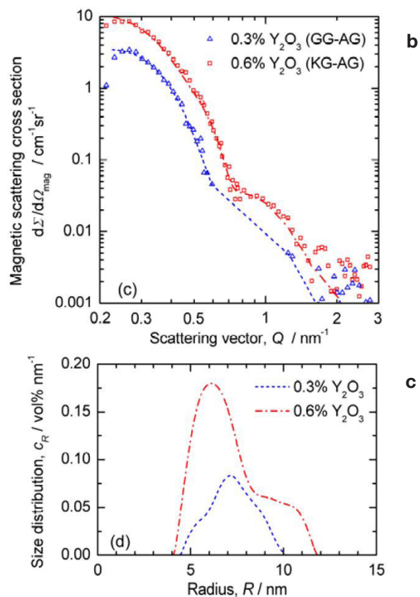
Figure 2: (a) The new 1.5T magnet mounted on KWS-1. (b) First SANS measurements on \text{Y}_2\text{O}_3 grains dispersed in steel. (c) From the scattering curves, the grain size distribution is determined.
