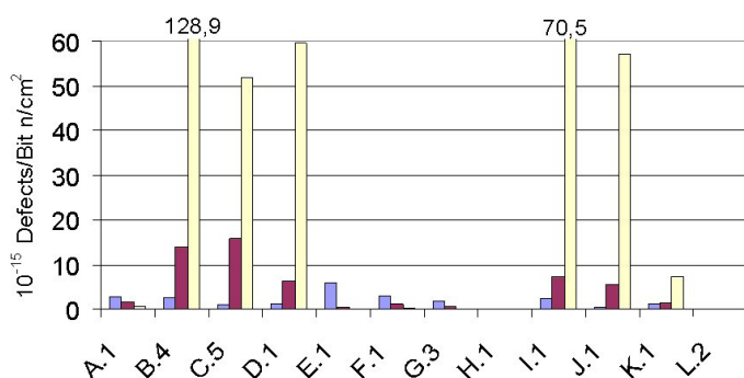
Figure 4: Comparison of the SEU defect trend of different SRAM devices exposed to varying kinetic energies of the neutrons. (yellow: low energy neutrons, red: thermal neutrons, blue: high energy neutrons).
